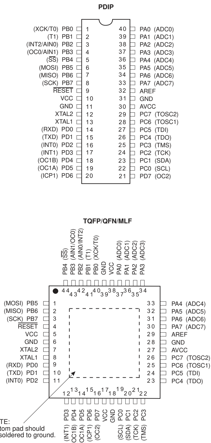
Figure 1-1. Pinout ATmega16A
