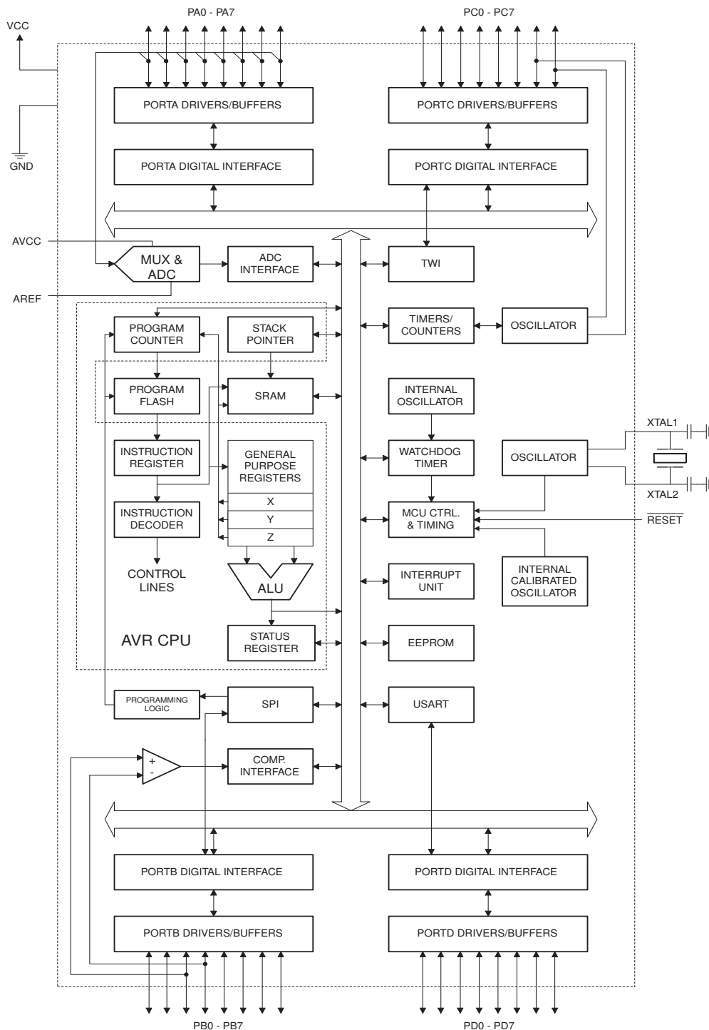
Figure 2-1. Block Diagram
